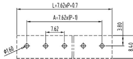
PCB Layout
