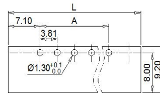
PCB layout for reference only
